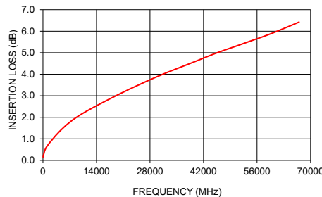
E67-1M-EMEM+ INSERTION LOSS
