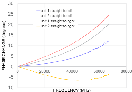
TYPICAL PHASE vs. FLEXURE*
