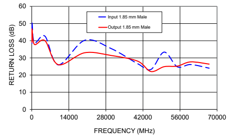
E67-1M-EMEM+ RETURN LOSS
