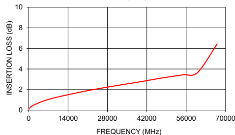
E67-2FT-EMEM+ INSERTION LOSS
