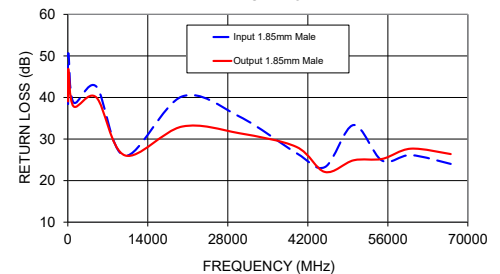
E67-2FT-EMEM+ RETURN LOSS
