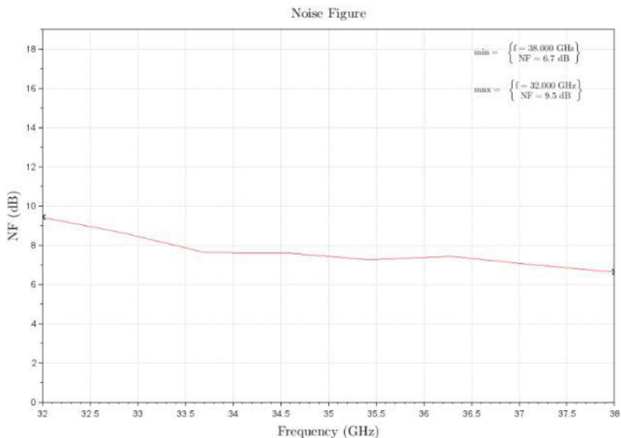
Figure 5: ERZ-HPA-3200-3800-40 Noise Figure
