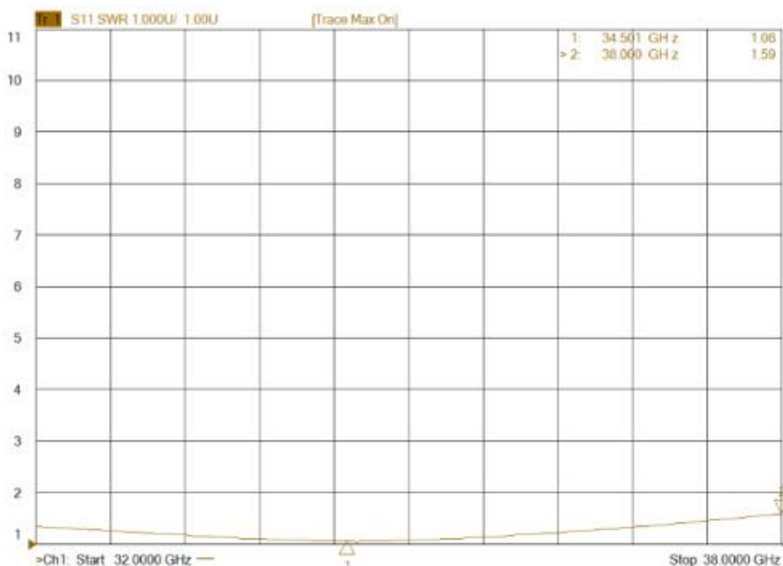
Figure 3: ERZ-HPA-3200-3800-40 VSWR IN
