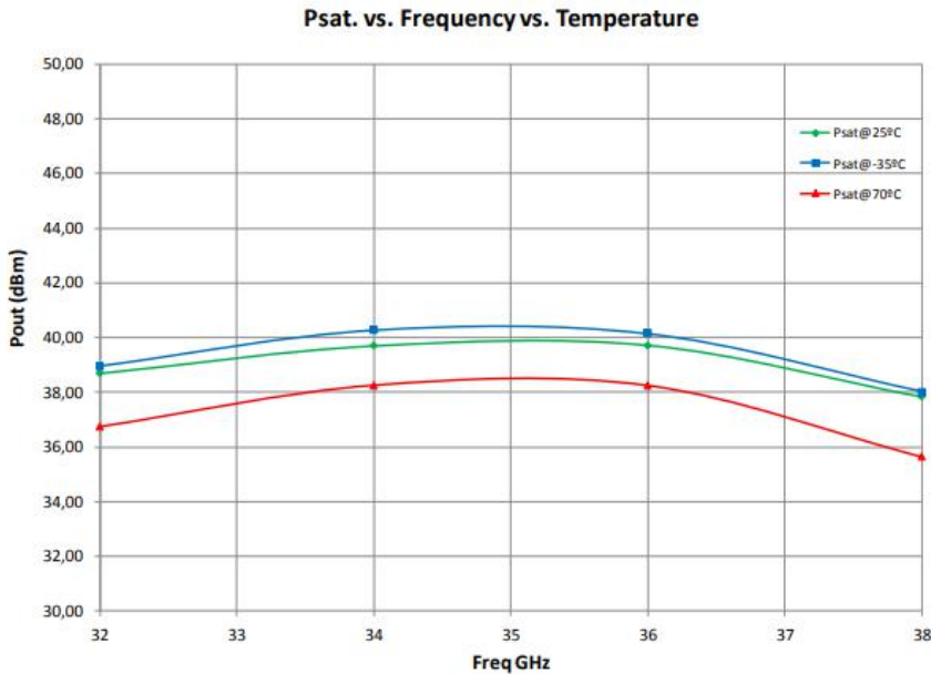
Figure 1: ERZ-HPA-3200-3800-40 Psat
