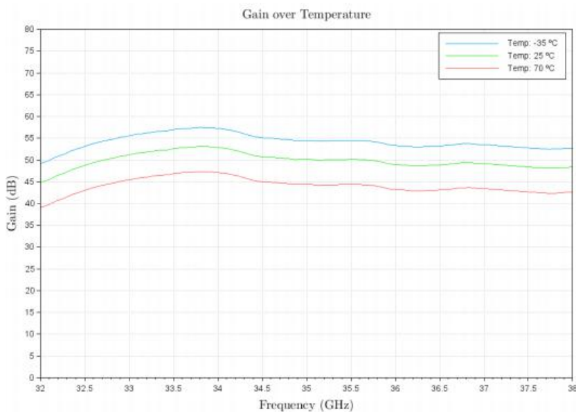
Figure 2: ERZ-HPA-3200-3800-40 Small Signal Gain
