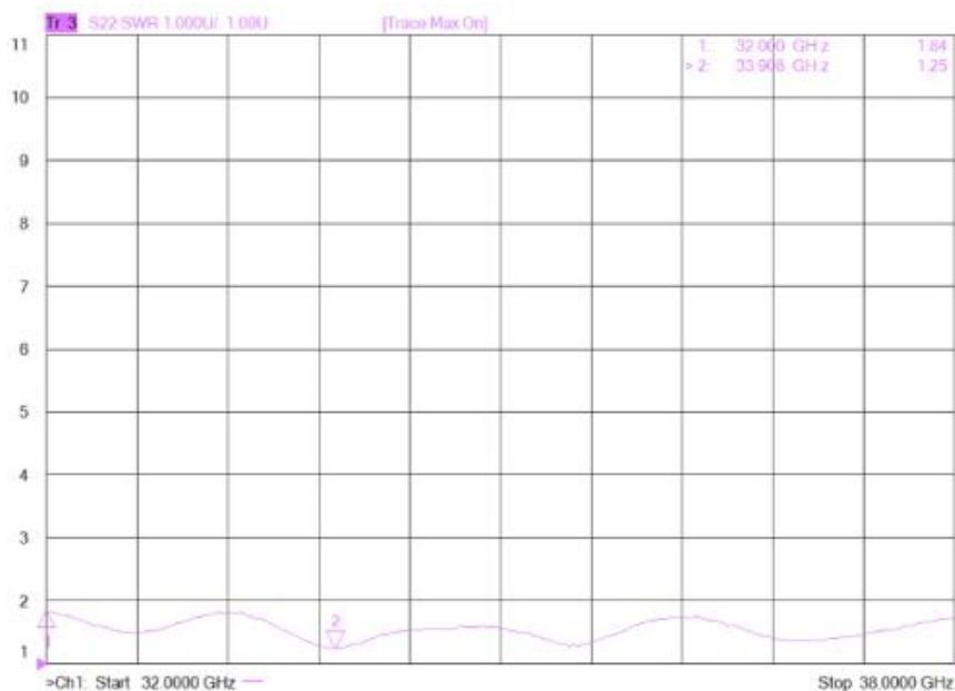
Figure 4: ERZ-HPA-3200-3800-40 VSWR OUT
