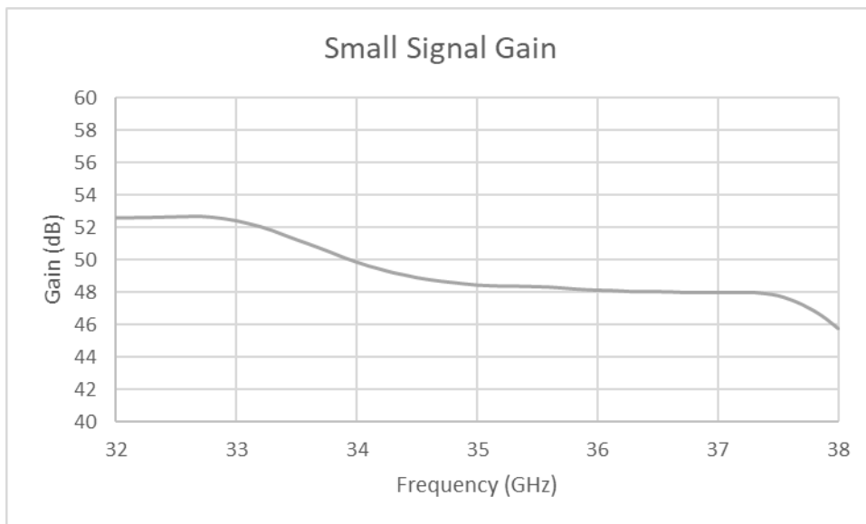
Figure 2: ERZ-HPA-3200-3800-40 Small Signal Gain
