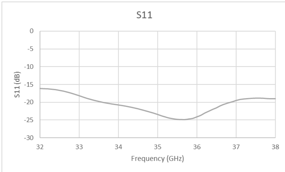
Figure 3: ERZ-HPA-3200-3800-40 S11
