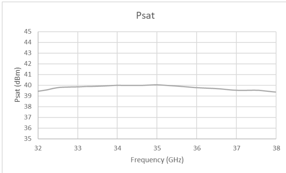
Figure 1: ERZ-HPA-3200-3800-40 P_{sat}
