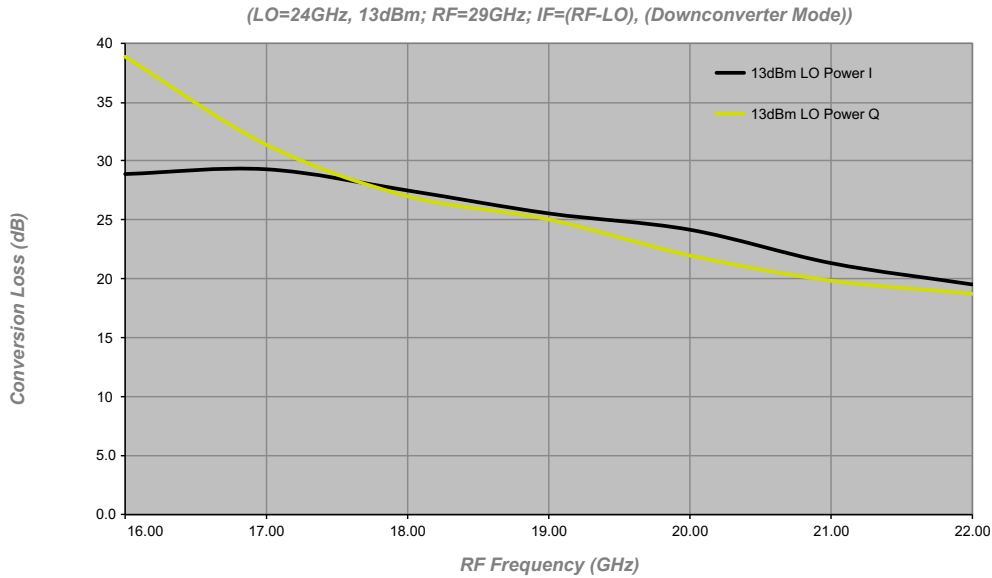
Figure 3 Conversion Loss (Image Band)
