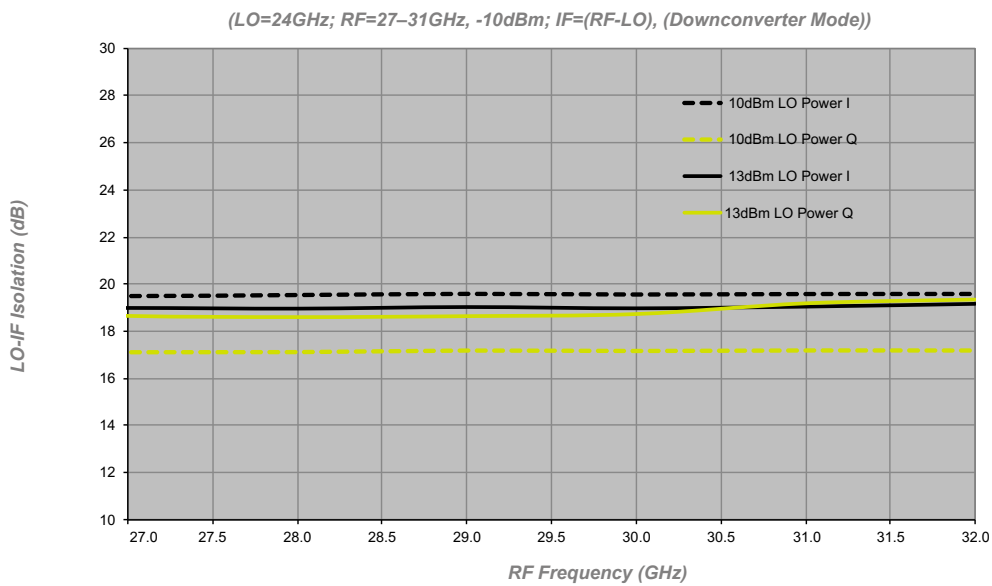
Figure 2 LO-IF Isolation
