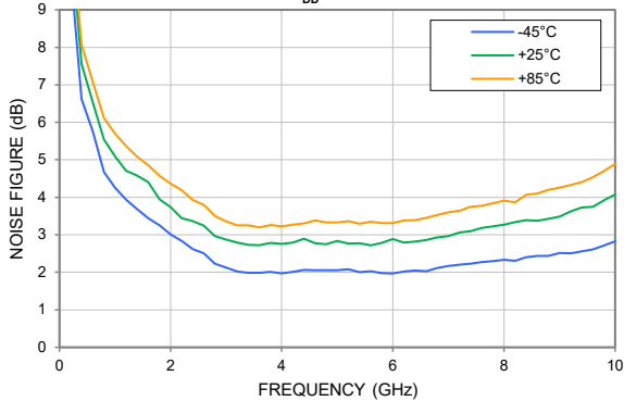
NOISE FIGURE vs. TEMPERATURE, V DD = +12 V
