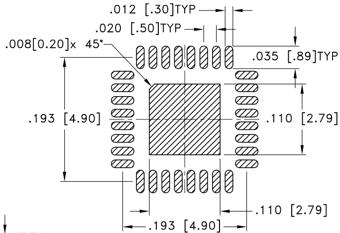
SUGGESTED LAYOUT FOR PCB LAND PATTERN (TOL ±.002)
