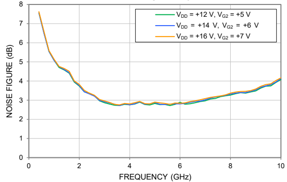
NOISE FIGURE vs. DEVICE VOLTAGE, TEMPERATURE = +25°C
