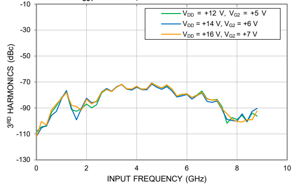
3 RD HARMONICS vs. DEVICE VOLTAGE, P OUT = +10 dBm, TEMPERATURE = +25°C
